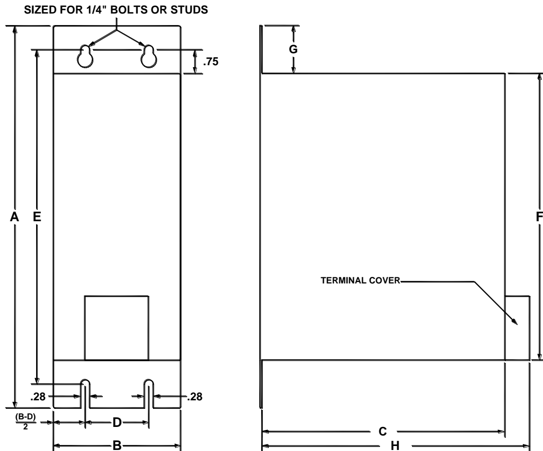
Figure 6-1: Bookshelf and Mini Chassis Dimensional Outline Drawing
