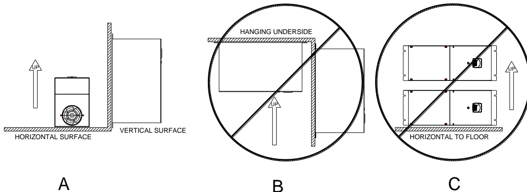
Figure 3-1: M3575R Mounting Orientation
