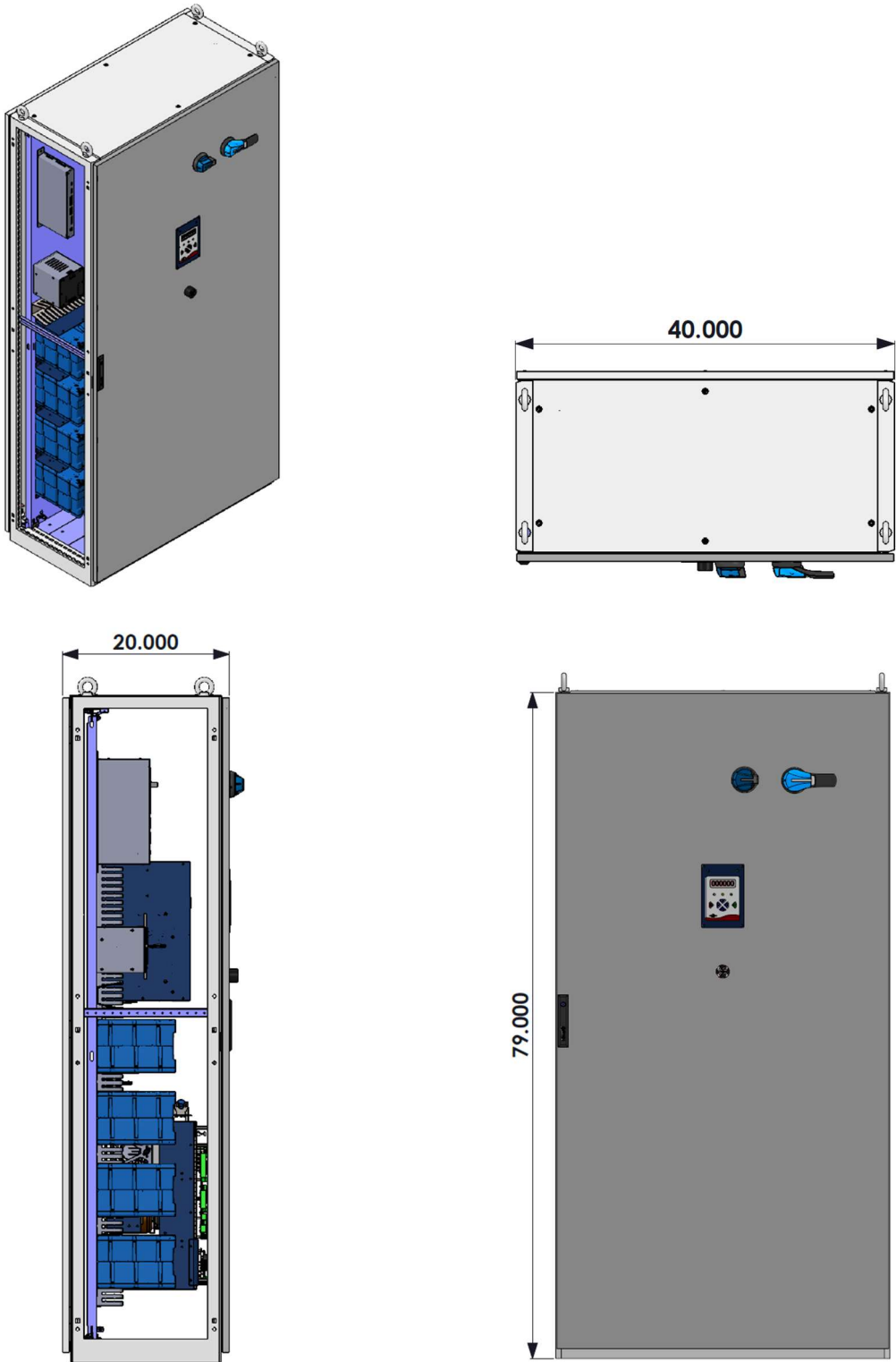
Figure 6-1: D82 Cabinet Dimensional Outline. 50KW
