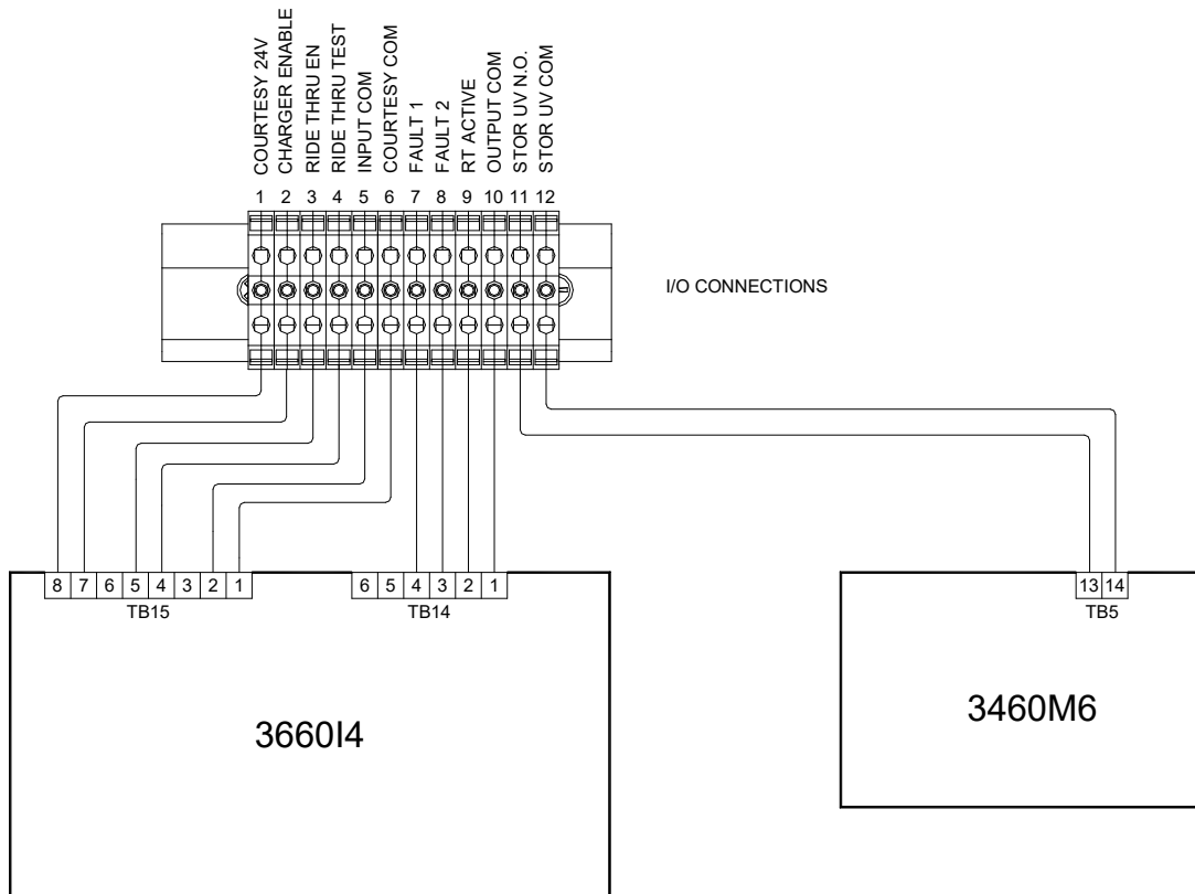
Figure 3-3: User I/O Connections with DD5 Interface Module
