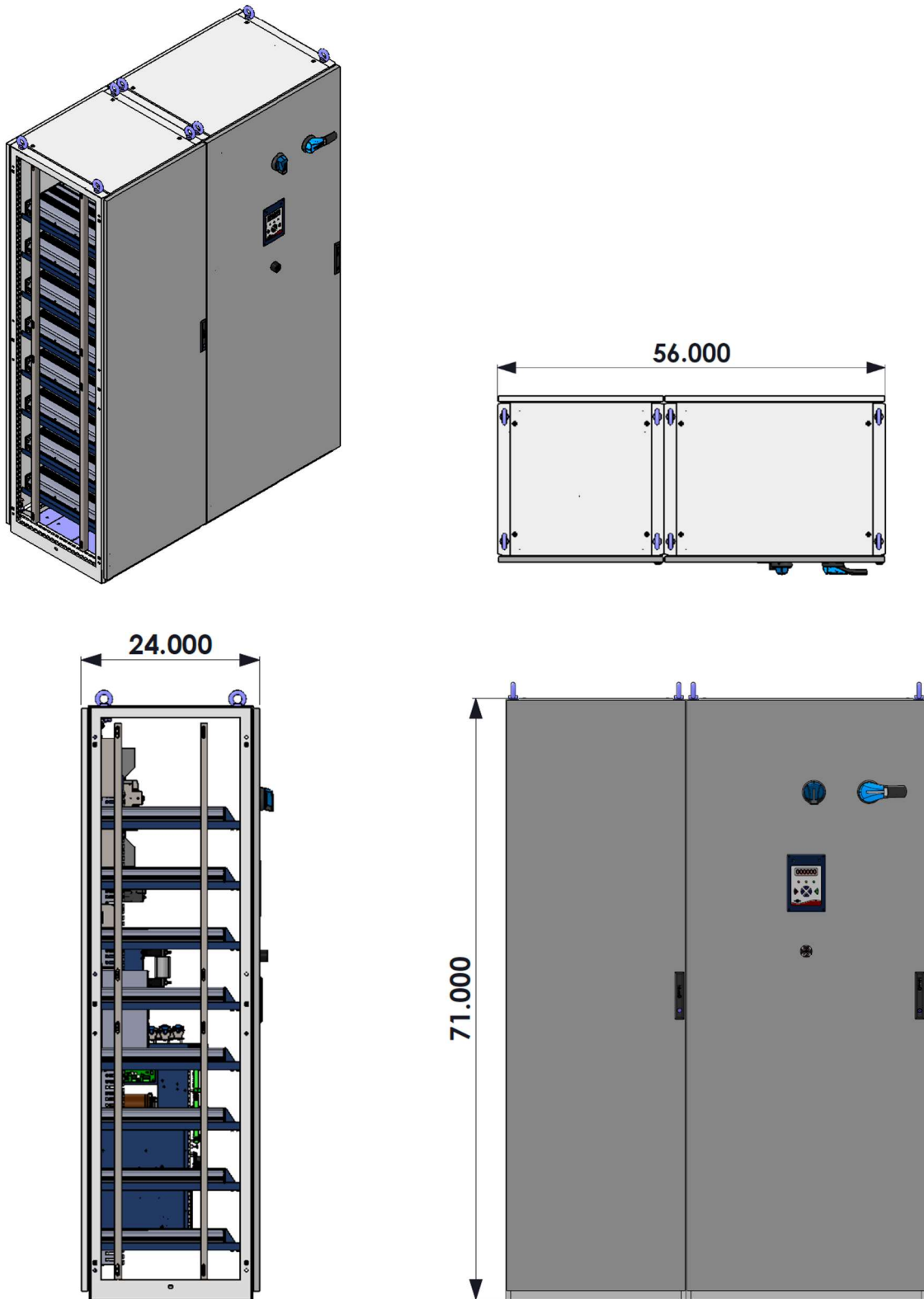
Figure 6-2: 75KW-100KW Cabinet Dimensional Outline
