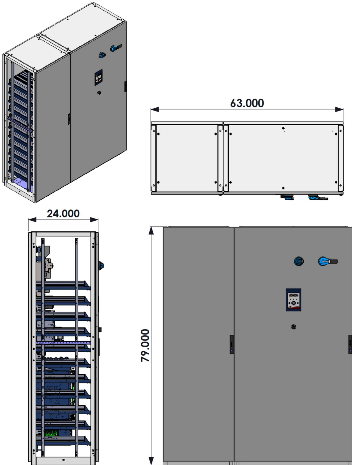
Figure 6-4: 250KW Cabinet Dimensional Outline
