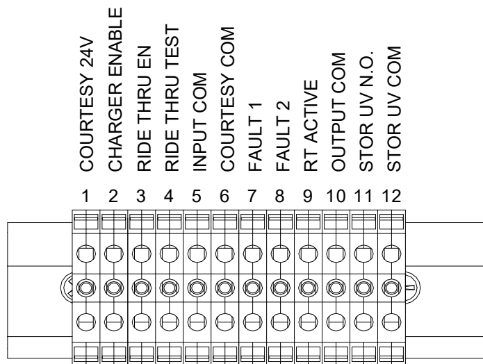
I/O CONNECTIONS
