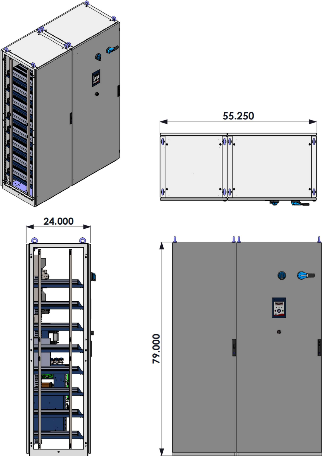
Figure 6-3: 150KW-200KW Cabinet Dimensional Outline
